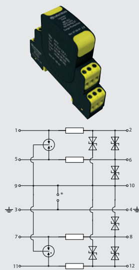
MP 2x2 GDT/Ad-Ad-Pg ST
