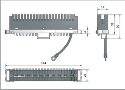
SSCT ground module LSA 2/10-ER38-rot
