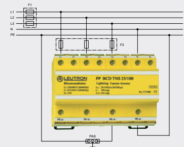
Combined arrester Type 1+2+3 PowerPro BCD at the LPZ transition point 0 A -2*
