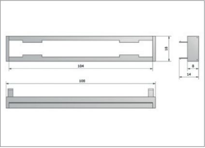
LSA – SSCT frame
