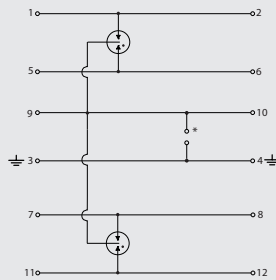
MP 2x2 GDT ST
