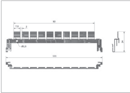
SSCT ground bar
