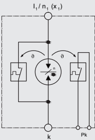
Basic circuit diagram
