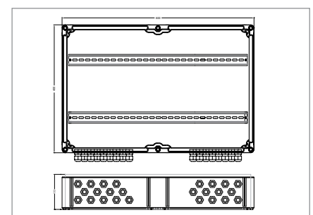
GAK 600 x 400 x 132 mm
