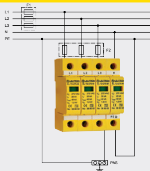
SPD Type 2 (class II), Spur wiring at the LPZ transition point 0B-1*
