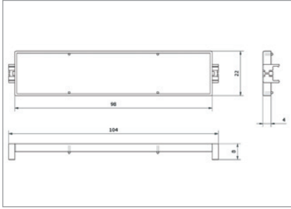
SSCT magazine cover
