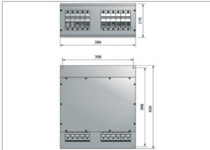
EPF, EMC Filter (three-phase) from 63 A
