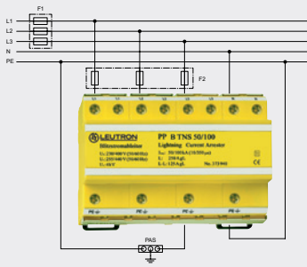
Lightning current arrester Type 1, PowerPro B at the LPZ transition point 0 A – 1*
