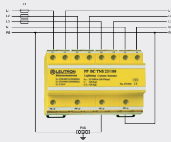
Combined arrester Type 1+2 (V wiring) PowerPro BC at the LPZ transition point 0 A -2*
