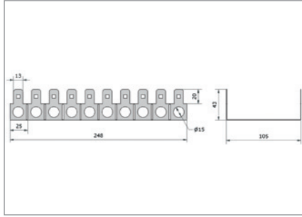
SSCT backmount frame
