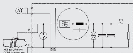
Basic circuit diagram
