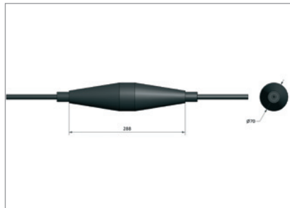
SGO 70QA and 350QA
