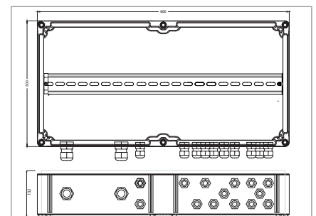
GAK 600 x 300 x 132 mm
