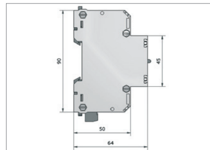
PP PV 800 and PP PV 1000
