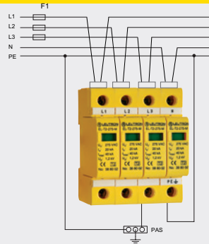
SPD Type 2 (class II), V wiring at the LPZ transition point 0B-1*
