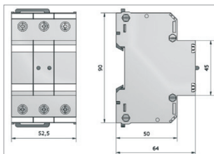
EnerPro 6A LED
