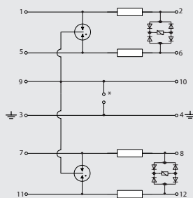
MP 2x2 HF ST
