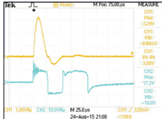
Surge Performance Data for the LP-DOE-1G
